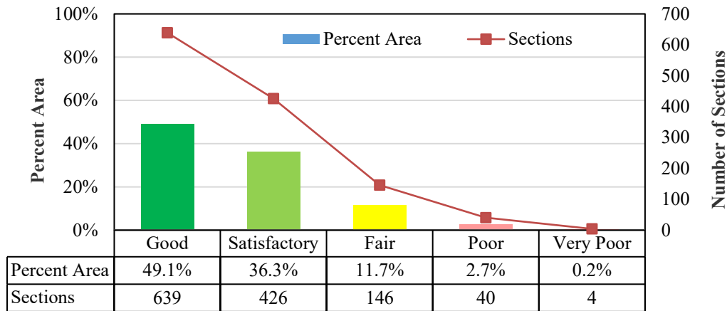
Figure 1 Overall Pavement Condition Distribution
