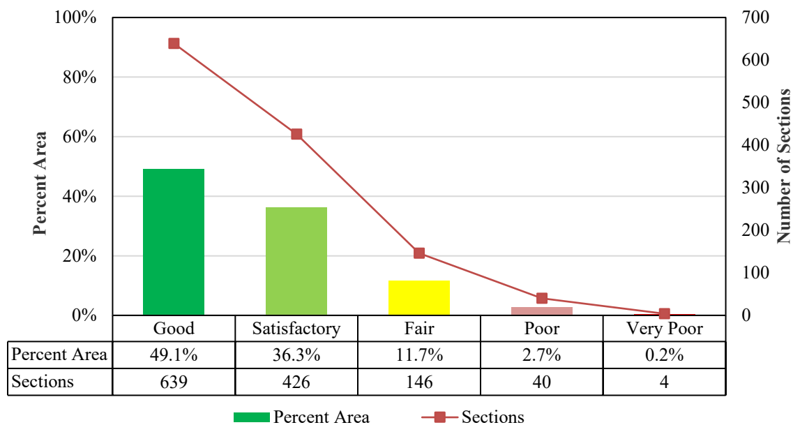
Figure 9 City's Overall Pavement Condition Distribution
